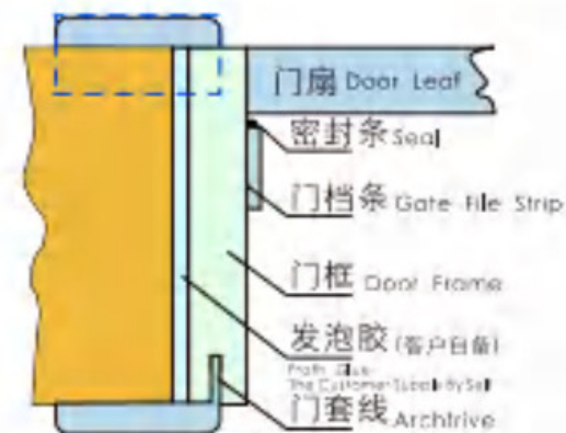
DIY组合门套安装示意 DIY Combination Suit Installation
